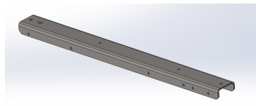
Outboard Support Rail (1):
